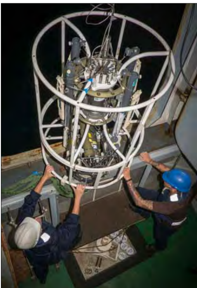
● Echo’s sailors prepare to launch a CTD probe into the Southern Indian Ocean at night
