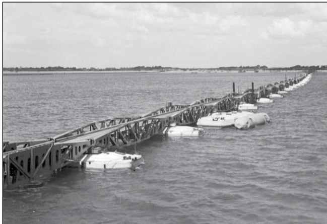
● Part of the Whale flexible roadway of a Mulberry Harbour, supported by Beetles
